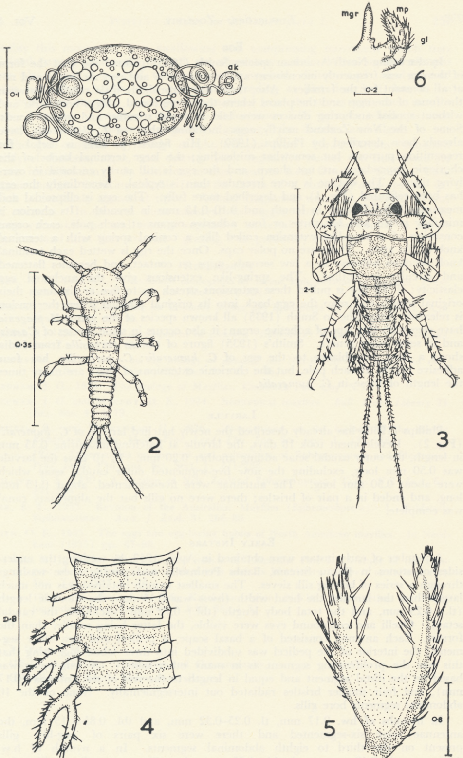
FIGS. 1-6.—Fig. 1—Lateral view of egg: e = chorionic extension, ak = adhesive knob. Fig. 2—Larvule (after Phillips 1930). Fig. 3—Young nymph. Fig. 4—Anterior abdominal tergites of a young nymph showing transition in gill structure. Fig. 5—Gill of last instar nymph. Fig. 6—Maxillary gill rudiment (mgr) attached to base of maxillary palp (mp) and galea-lacinia (gl) in a young nymph. All measurements in mm. Camera lucida.
