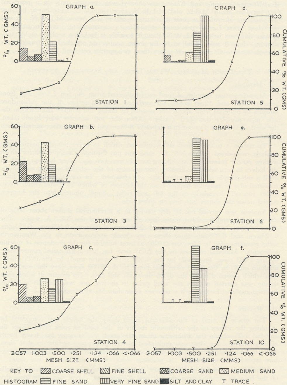
FIG. 7.—Histograms and cumulative curves of grade fractions of the surface sand at representative stations on the main beach.
