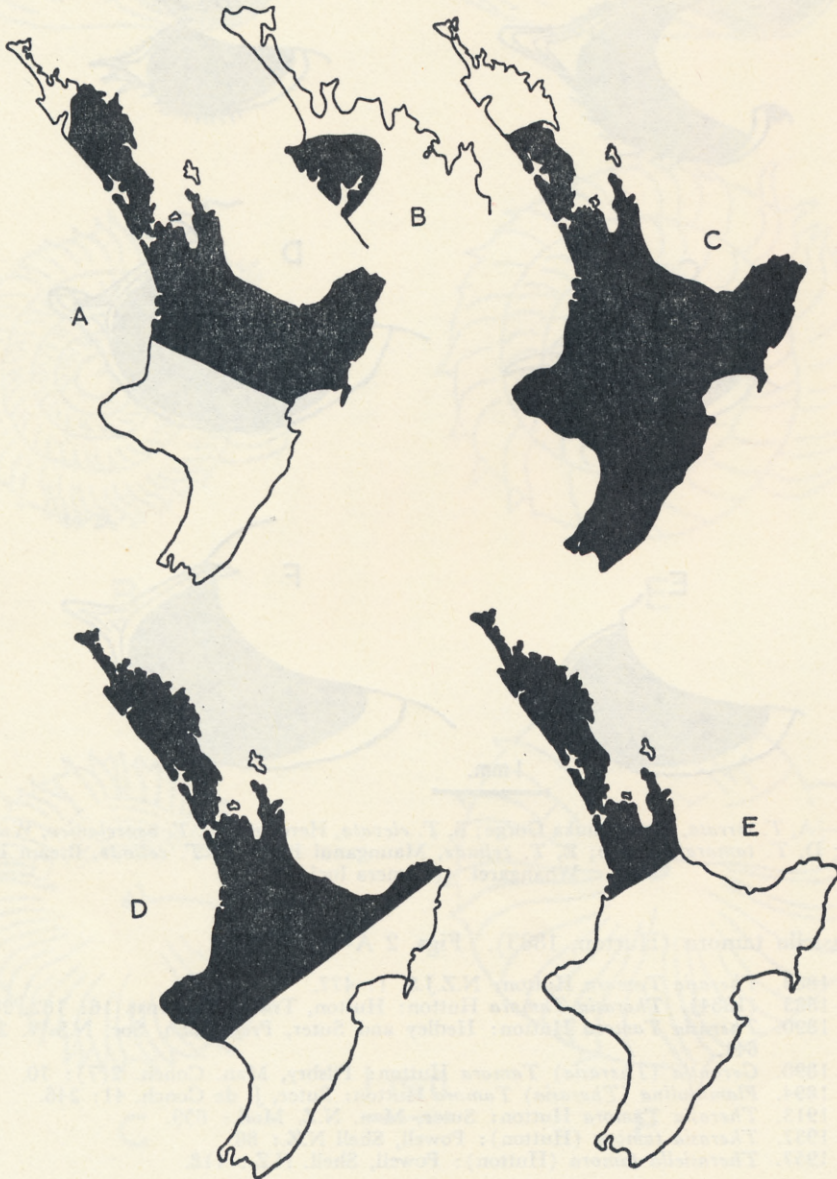
FIG. 5.—Distributions of the species are indicated by the black zones. A, T. serrata ; B, T. elevata ; C, T. neozelanica ; D, T. celinde ; E, T. tamora .
