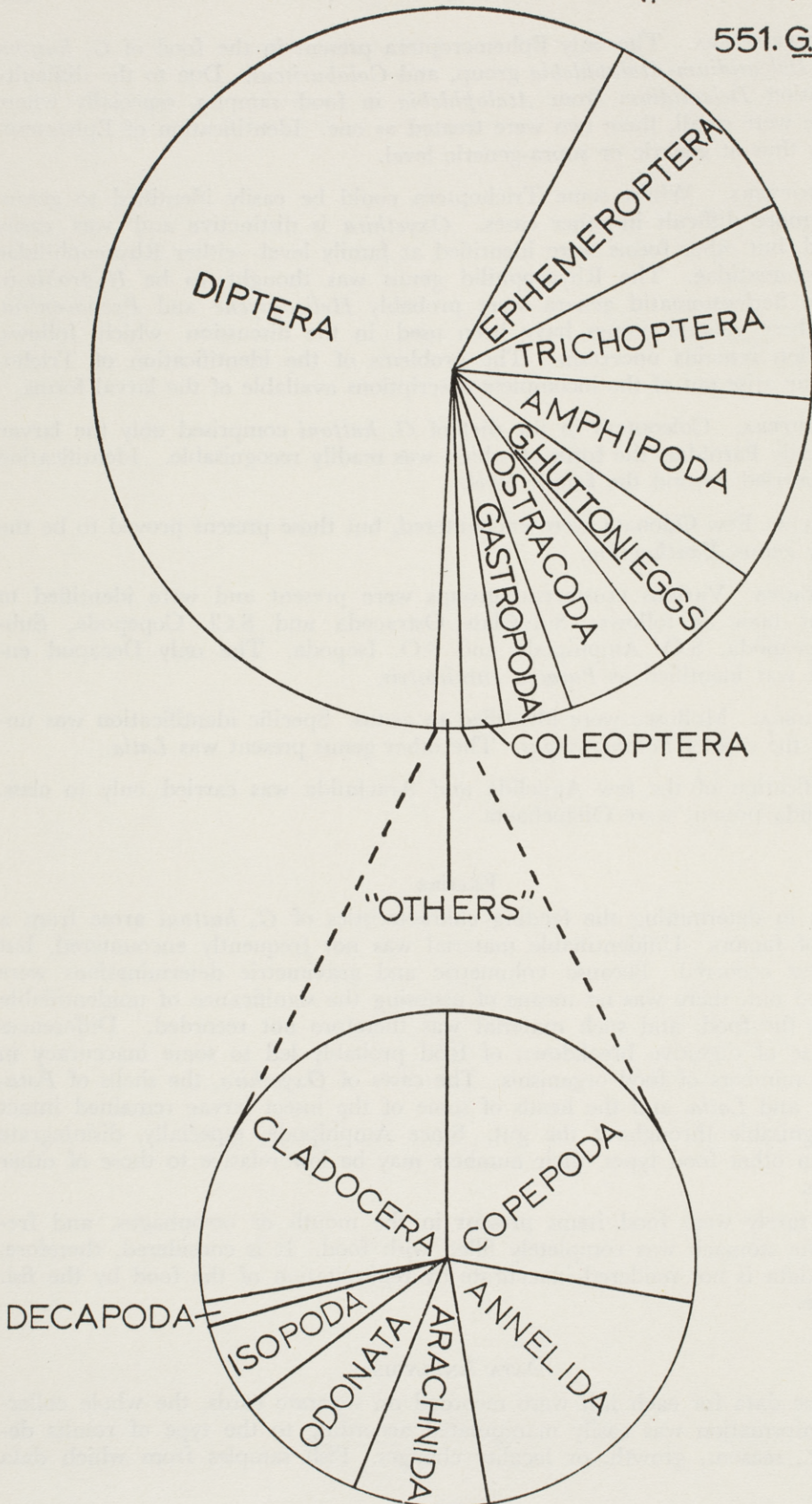
FIG. 2.—General composition of diet of G. huttoni .
