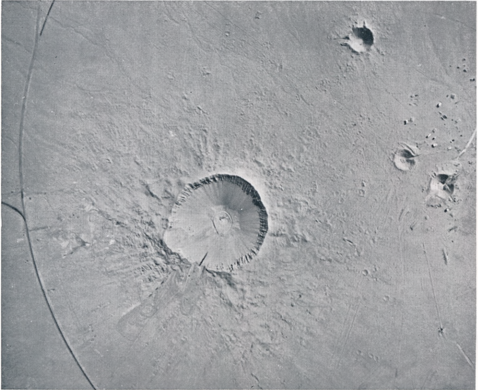
FIG. 3.—Sedan Crater, a crater resulting from a nuclear explosion on earth.
