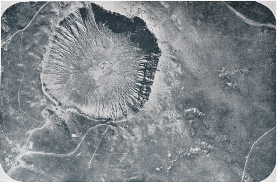
FIG. 4.—Winslow Crater, resulting from a meteoric impact on earth.
