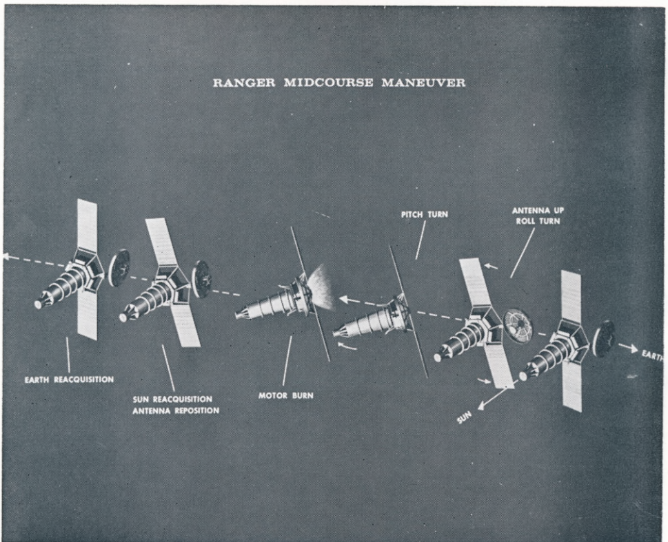
FIG. 12.—Ranger mid-course manoeuvre.
