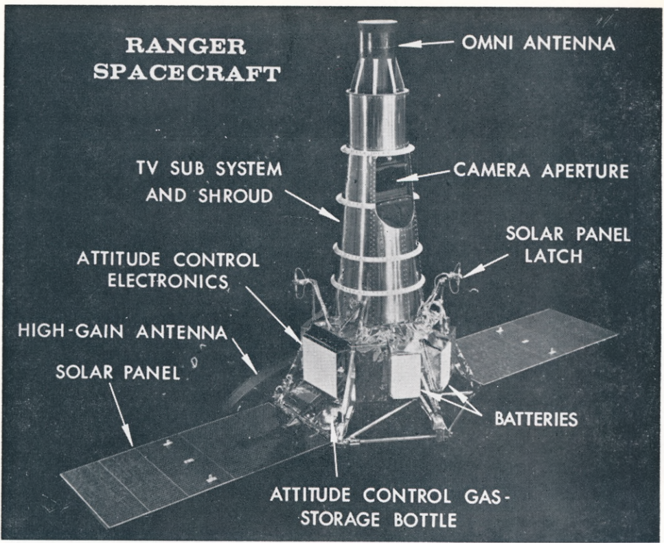
FIG. 11.—Ranger Spacecraft.
