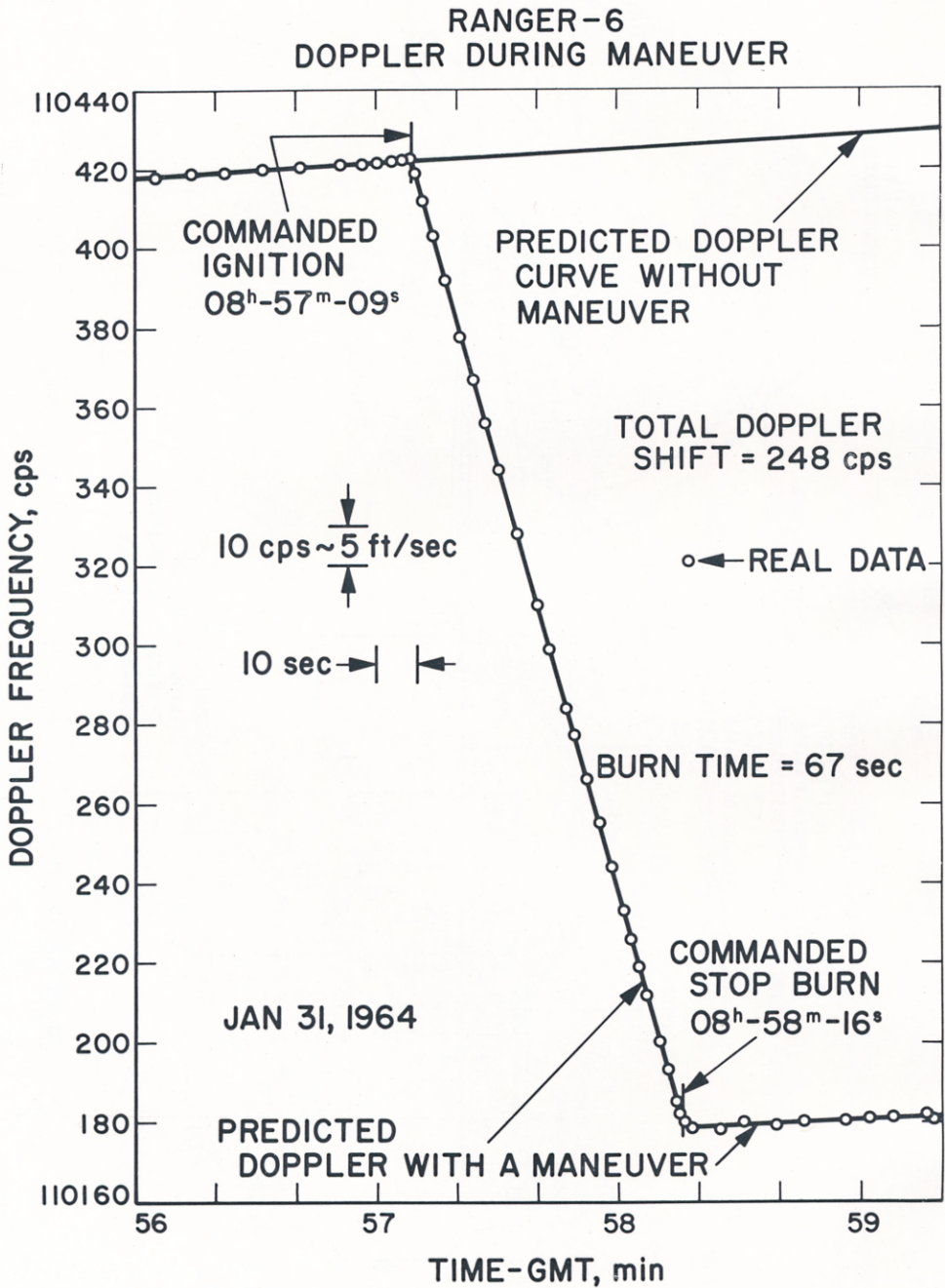
FIG. 17.—Ranger VI Doppler during manoeuvre.
