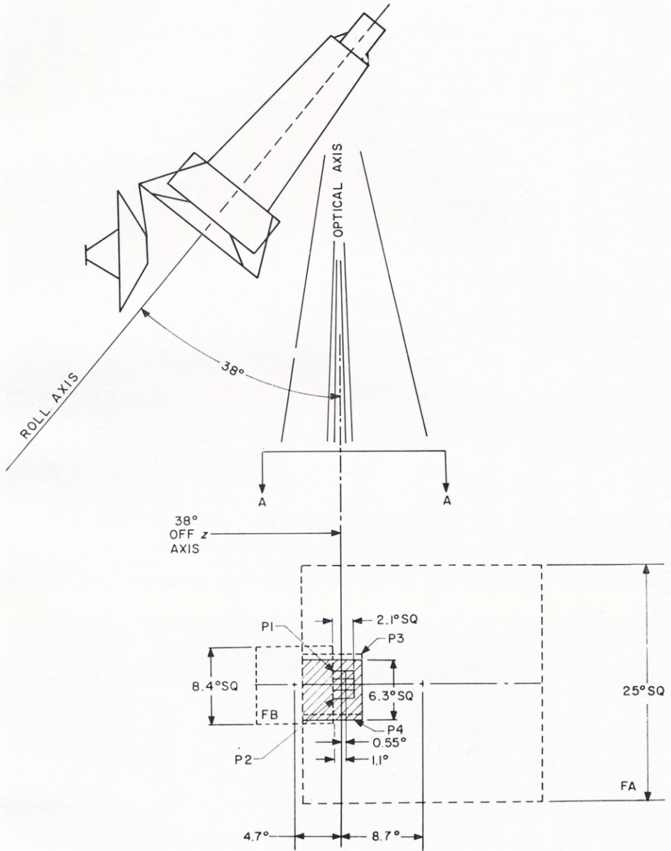
FIG. 16.—Optical axes orientation field of view.
