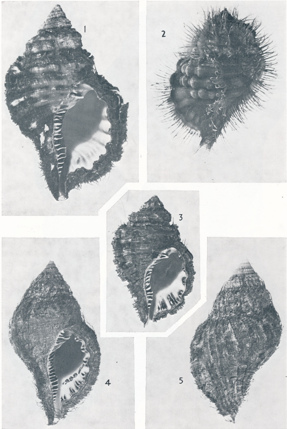
FIG. 1.— Septa (Monoplex) parthenopea echo (Kira), Japan (data unknown), pres. Dr T. Kotaka; Victoria University Geology Department, VM. 817; 112.5 × 65.4mm. Fig. 2.— Septa (Monoplex) parthenopea parthenopea (Salis), Darch Pt., Whangarei Heads, New Zealand; Dominion Museum spirit colln.; 94 × 84mm (incl. periostracum). Fig. 3.— Septa (Monoplex) parthenopea parthenopea (Salis), Narooma, New South Wales, Australia, pres. T. A. Garrard; Victoria University Geology Department, VM. 818; 79.7 × 47.4mm. Figs. 4, 5.— Septa (Monoplex) parthenopea keenae n.subsp., paratype, California Academy of Sciences loc. 38865, Academy Bay, Santa Cruz Id., Galapagos Is., Mrs C. Angermeyer, 1964; 85.7 × 43.1mm.
