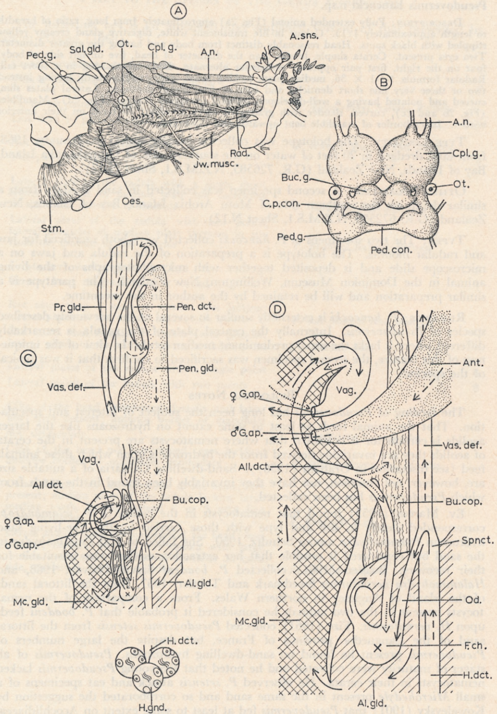
FIG. 3.— P. mortoni n.sp. A. Dissection of buccal mass and nerve ring from right side. B. Nerve ring reconstructed from sections. C. Reconstruction of the reproductive system. The various organs are shown in approximately correct proportions except the gonad in which the spatial relationships have been altered for clarity. D. An enlarged diagram of the main ducts of the reproductive system showing the direction of travel of the reproductive products; solid arrows, ova; dashed arrows, autosperms; dotted arrows, allosperms. For abbreviations see Fig. 5.
