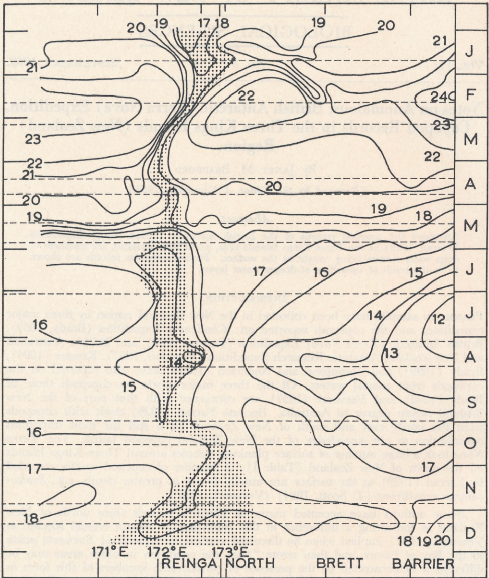
FIG. 1.—Surface temperature (°C) plotted as a function of position and time along the commercial coastal passage from Auckland northward through the Hauraki Gulf to North Cape, thence westwards to Sydney. Prominent geographical features are shown as abscissae and the months of the year as ordinates. Horizontal broken lines show the position of thermograph records used to construct this diagram (Garner, 1961).
