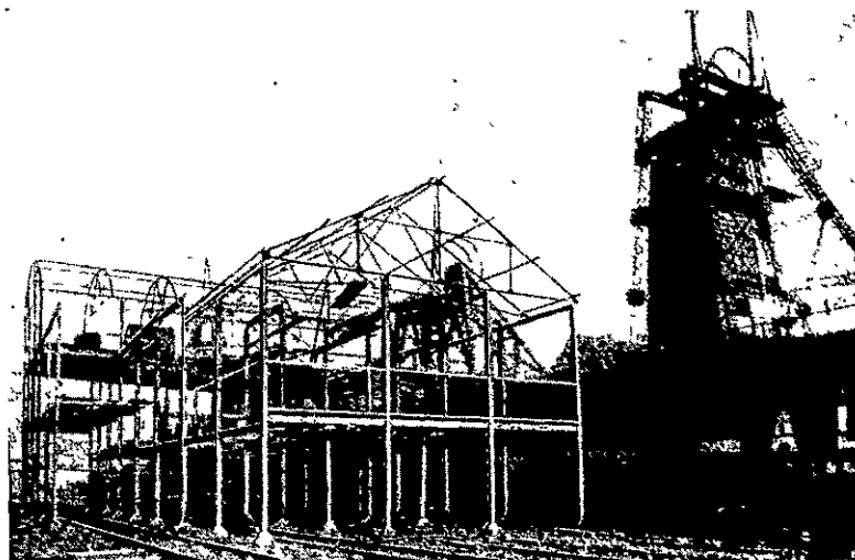
COMPLETE COAL SCREENING PLANT DURING ERECTION IN SOUTH WALES.
