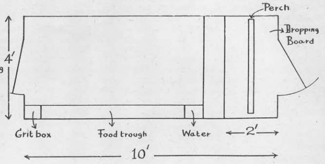
PLAN
