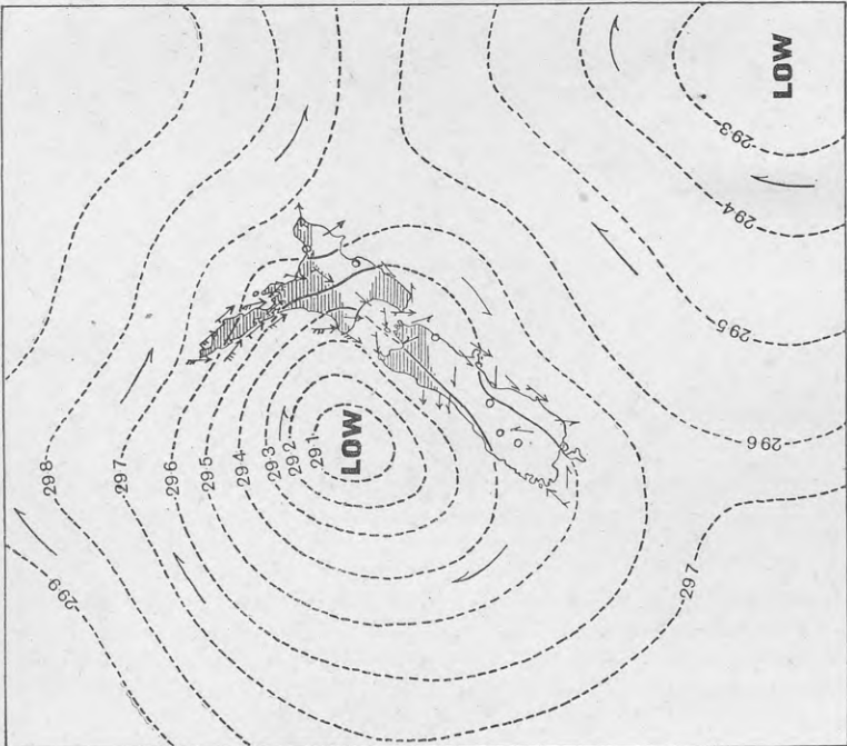
Fig. 11.—Weather chart, 16th December, 1913. Cyclone centred west of Farewell Spit.
