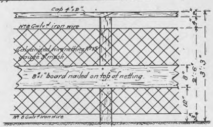
Elevation of Fence, Height 3'3"
