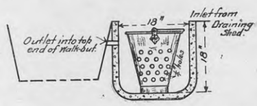
Settling Well for Drainage from Draining Shed. (18" x 18")
