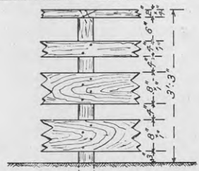
Alternative Type of Fence.
