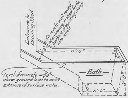
SMALL SHEEP DRAFTING, DIPPING, AND SHEARING PLANT.
