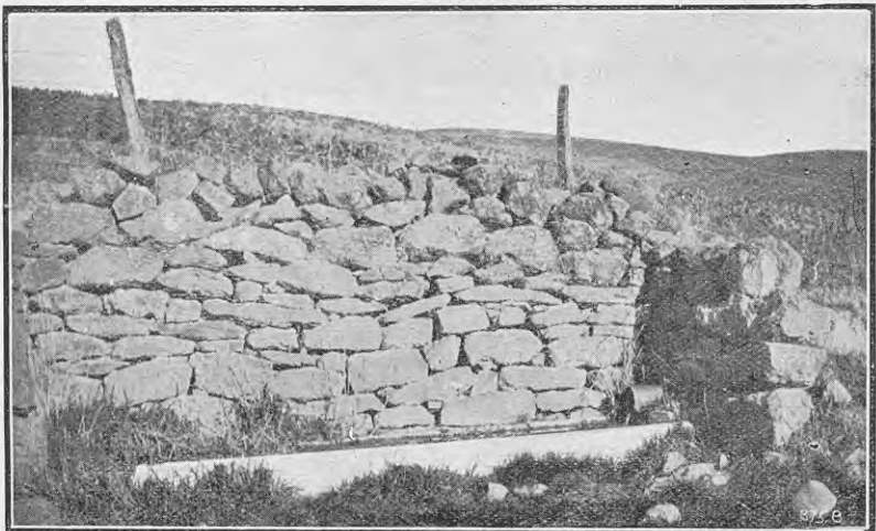
WELL-BUILT-UP WALL WITH PROTECTIVE NETTING AT BACK.
