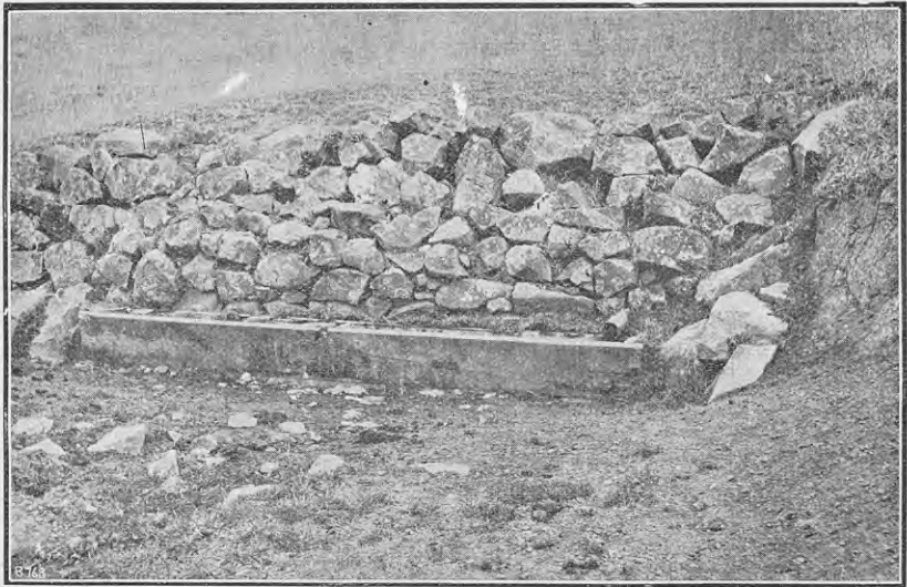
A GOOD TROUGH OF SIMPLER WALL-CONSTRUCTION.
