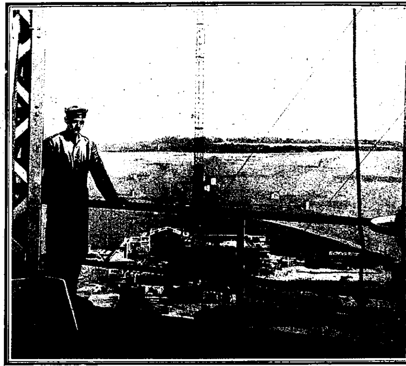
WIRELESS TELEGRAPHY AT A GERMAN STATION. The station of the Wireless Telegraphy Society at Nauen, in Germany, is able to send and receive telegrams from a distance of 10,000 miles. Our illustration shows an aspect of the southern tower, which measures 260 metres.
