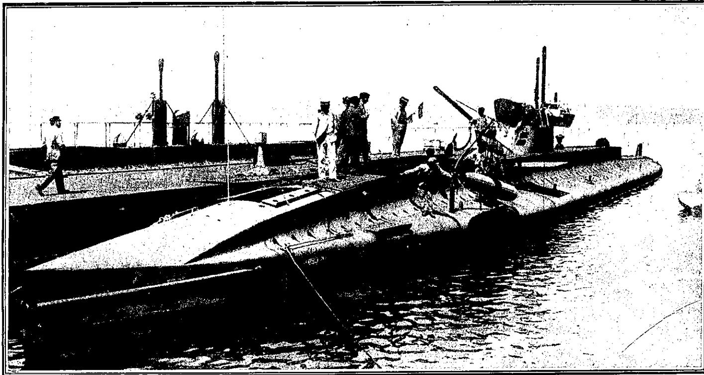
PLACING TORPEDOES IN THE FRENCH SUBMARINE XIPHIA.
