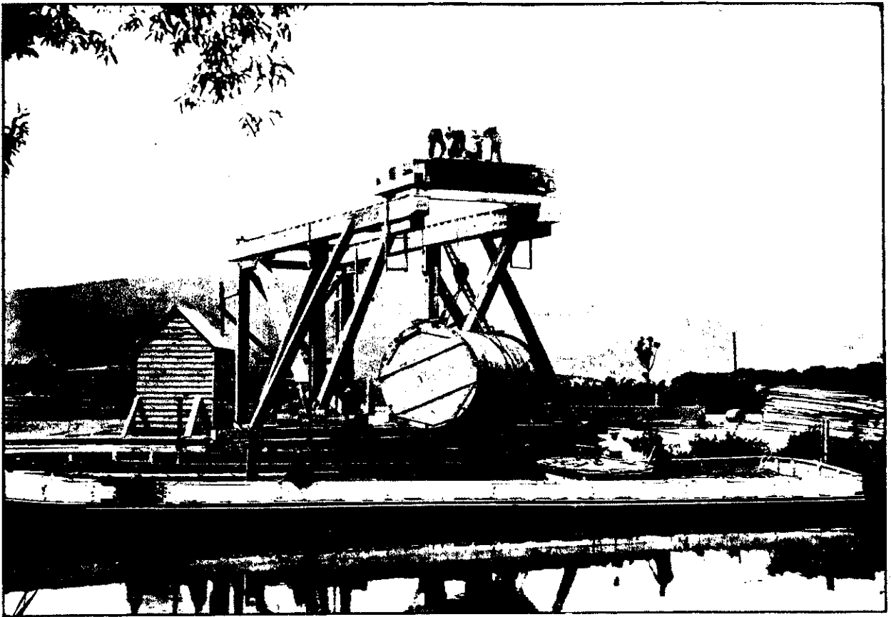
LANDING THE NEW CYLINDER FOR THE PUMPING ENGINE, WAIHI MINE. The largest and heaviest cylinder in the world. 16 feet long, 10 feet 6 inches diameter. Weighs 22 tons.
