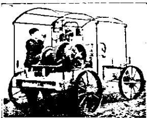
4 H.P. "UNION" OIL ENGINE AND PUMP.
