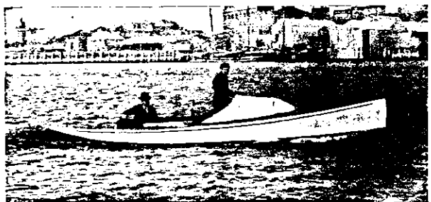
TITI. Fitted with 1 1/2 H.P. Hercules Engine. Length 23ft; Beam 5ft 6in; Draught, 1ft 6in. Built for Mr. Hughes, Picton, by Messrs. Bailey and Lowe.
