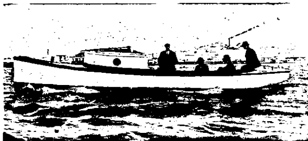
MARORO. Fitted with a 3 H.P. Hercules Engine. Length 30ft; Beam 7ft 6in. Built for F. W. Newton, Kawhia, by Messrs. Bailey and Lowe.
