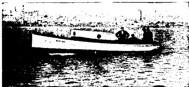
FARINA. Fitted with 5 H.P. Hercules Engine. Speed 3 miles. Length 30ft; Beam 7ft 6in. Built for Messrs. Rohrlach and Huxley, Thames, by Messrs. Bailey and Lowe.
