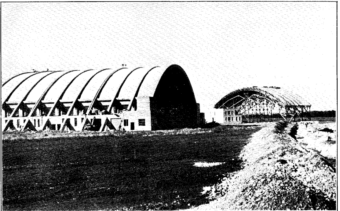
NO. 1 MAIN HANGAR. ADMINISTRATION BUILDING IN BACKGROUND; FALSEWORK BEING MOVED TO POSITION IN NO. 2 HANGAR.
