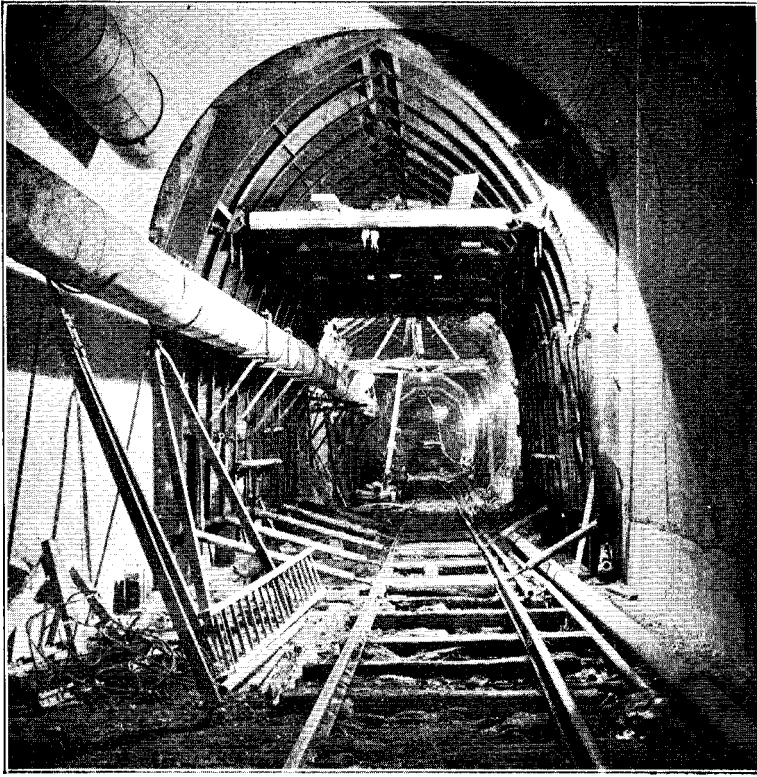
WAIKOURA TUNNEL, NORTH END. VIEW SHOWING STAGES OF CONSTRUCTION: TIMBERING IN BACKGROUND; STEEL FORMWORK IN MIDDLE DISTANCE, AND FINISHED LINED TUNNEL IN FOREGROUND.
