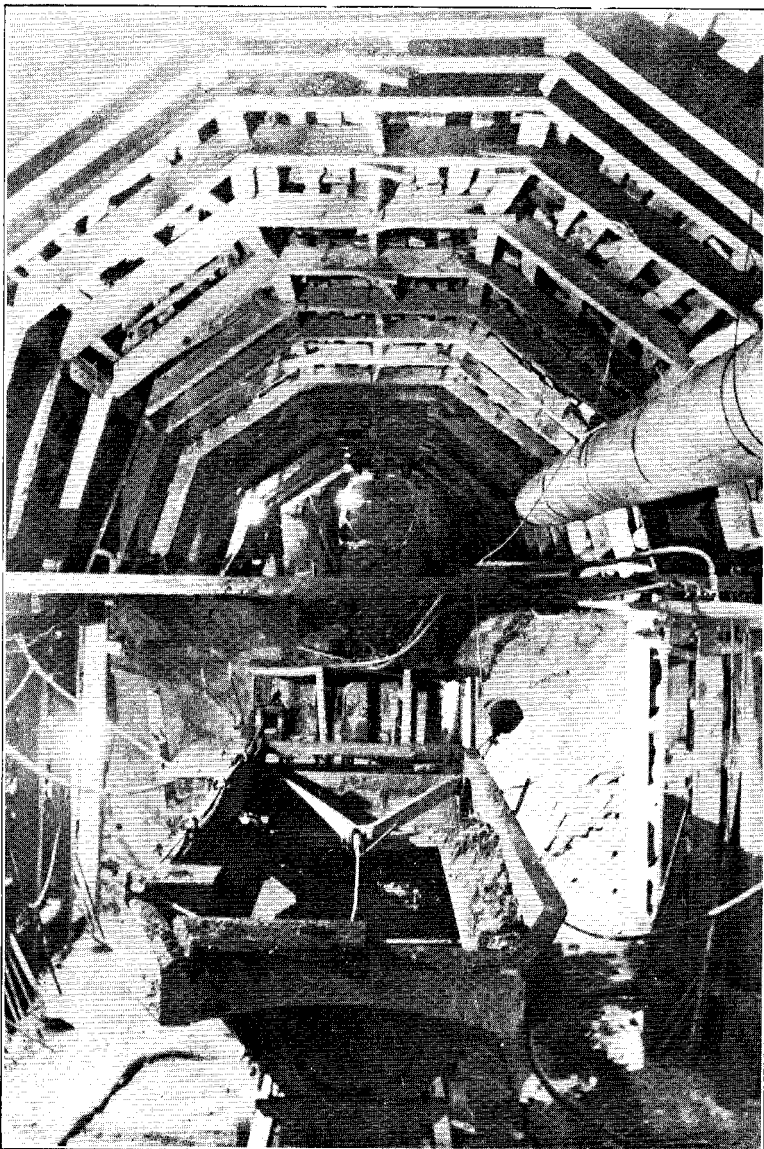
WAIKOURA TUNNEL, SOUTH FACE. VIEW SHOWS TIMBERING AND MECHANICAL MUCK-SCRAPER, GIBBORNE-NAPIER RAILWAY.
