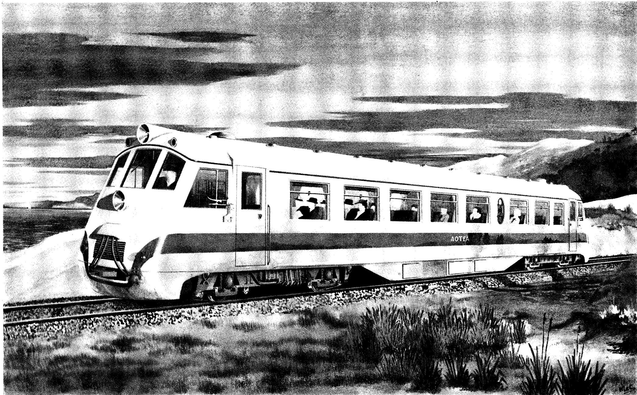
“AOTEA,” STANDARD TYPE OF RAIL-CAR FOR USE ON MAIN LINES AND FOR LONG DISTANCE RUNNING. Length, 66 ft.; Seating capacity, 52; Horse-power, 240; Weight (loaded), 32 tons.
