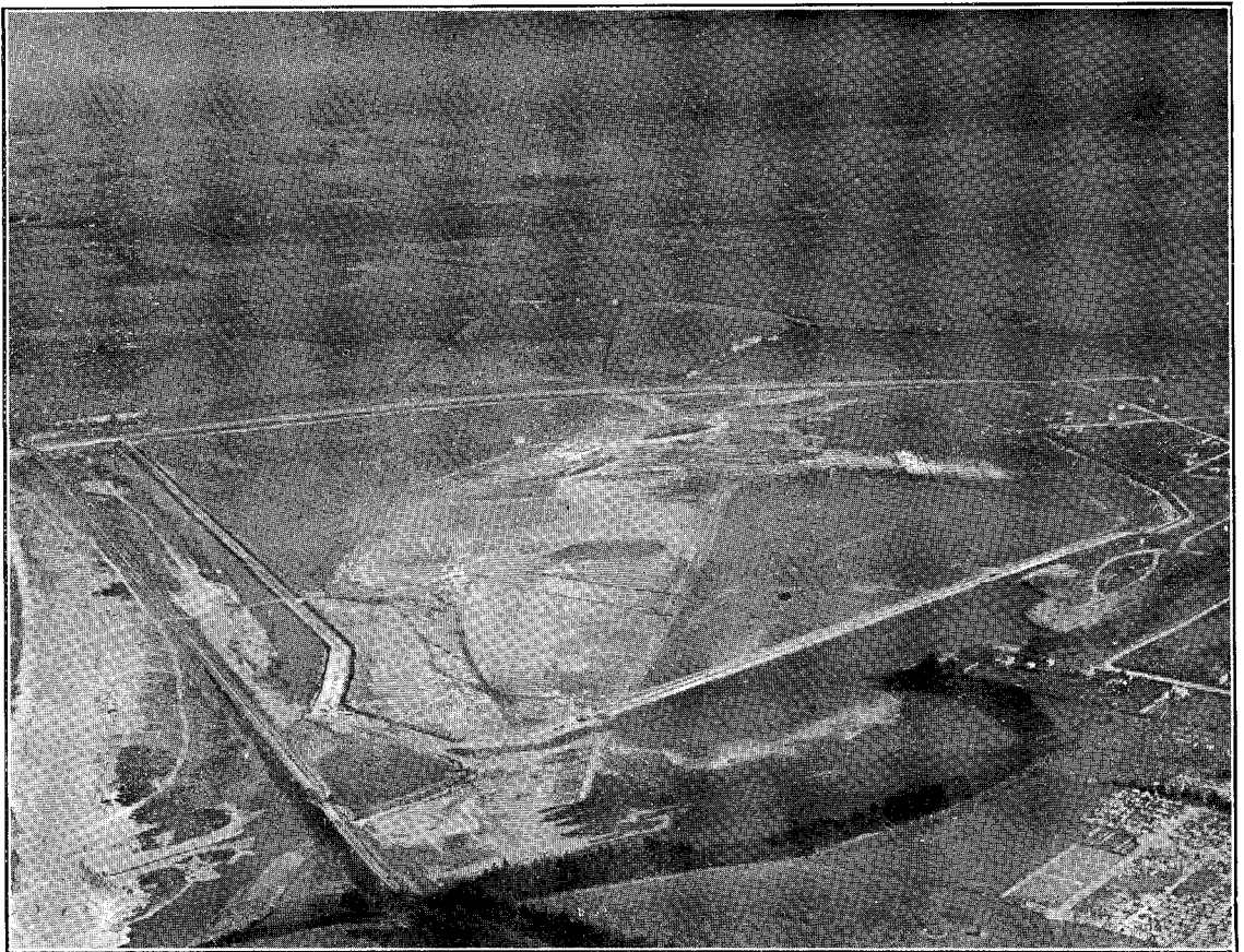
AERIAL VIEW SHOWING DRAINAGE AND RE-GRADING IN PROGRESS. SALTWATER CREEK AERODROME, TIMARU.
