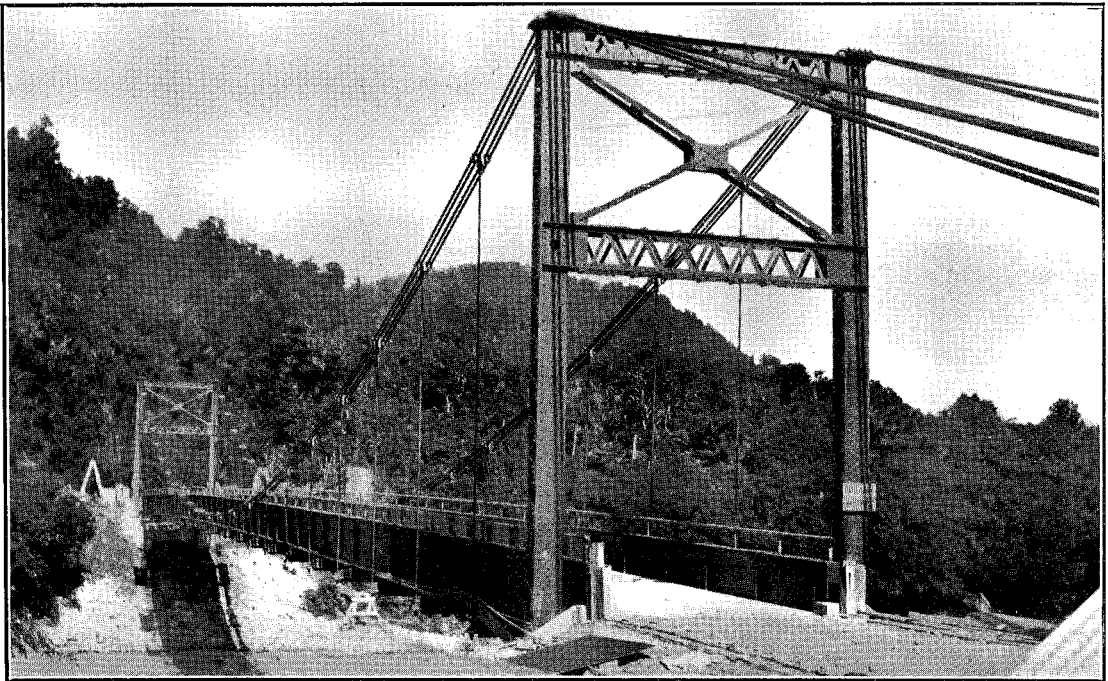
SUSPENSION BRIDGE, 264 FT. SPAN, 10 FT. 6 IN. ROADWAY, CONCRETE DECK. COOK RIVER BRIDGE. MAIN SOUTH ROAD, WESTLAND.
