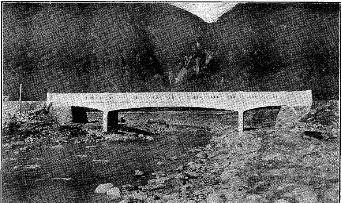
ONE 70 FT. AND TWO 19 FT. SPANS, 12 FT. ROADWAY; CONTINUOUS HOLLOW BOX GIRDERS OF REINFORCED CONCRETE.
