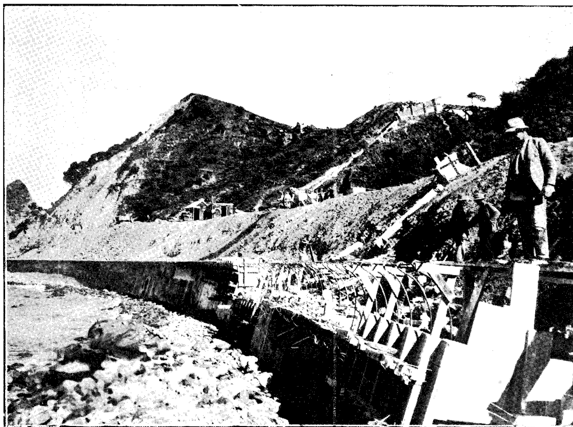
SEA-WALL IN COURSE OF CONSTRUCTION, WAIKOKOPU BLUFFS.
