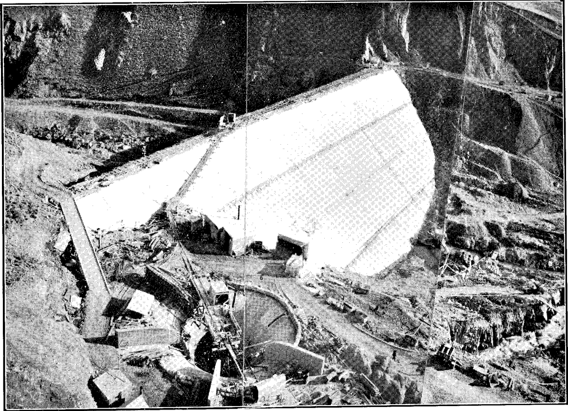
MANHERIKIA FALLS DAM, NEARING COMPLETION.—SHAFT SPILLWAY IN FOREGROUND. OMAKAU IRRIGATION SCHEME.
