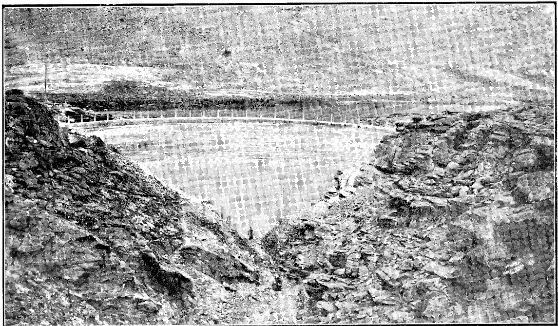
EARNSCLEUGH IRRIGATION SCHEME.—CONROY'S CREEK DAM.
