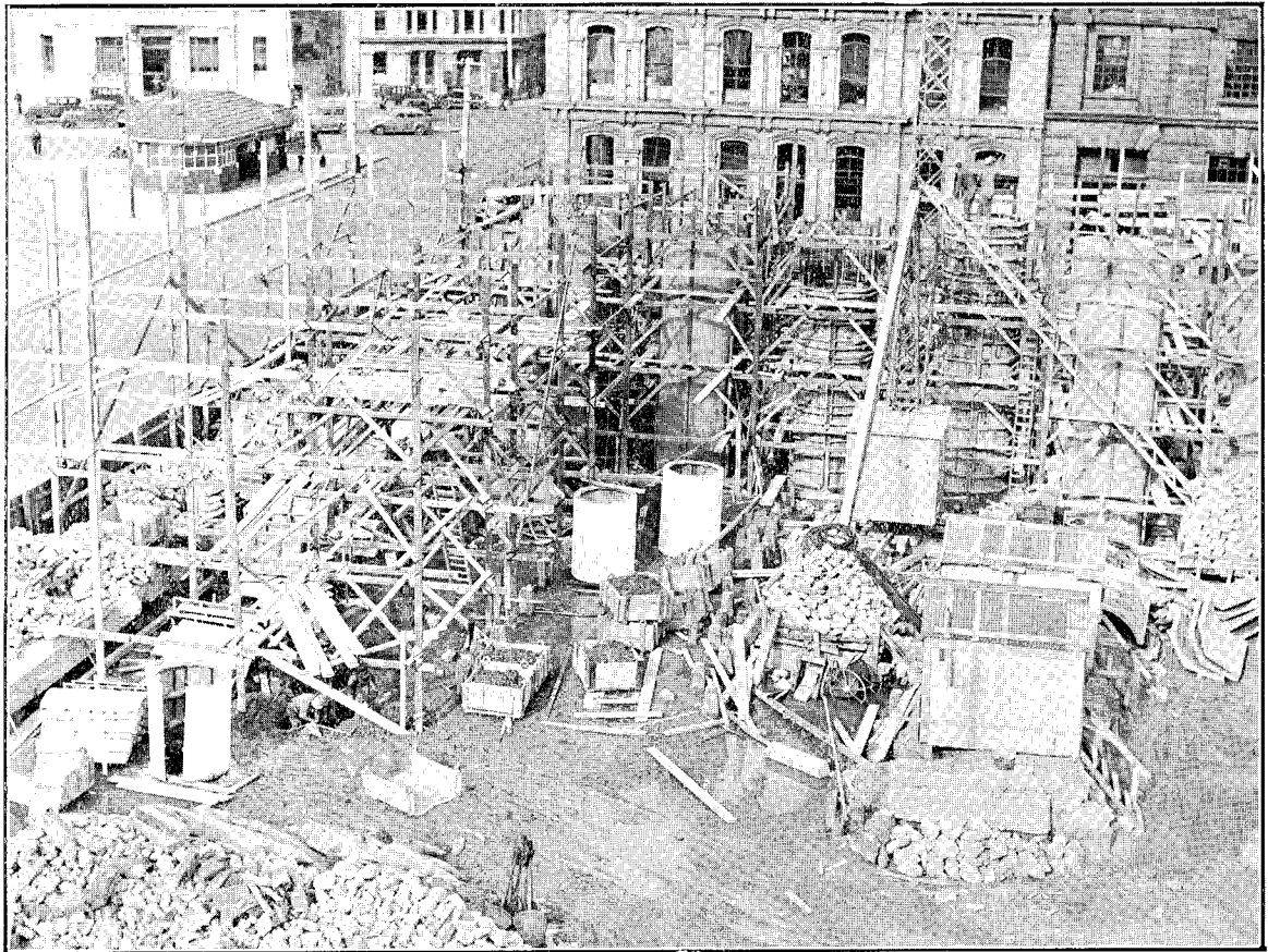
CAISSONS FOR FOUNDATIONS BEING CONSTRUCTED AND SUNK. GOVERNMENT LIFE INSURANCE BUILDING, WELLINGTON.
