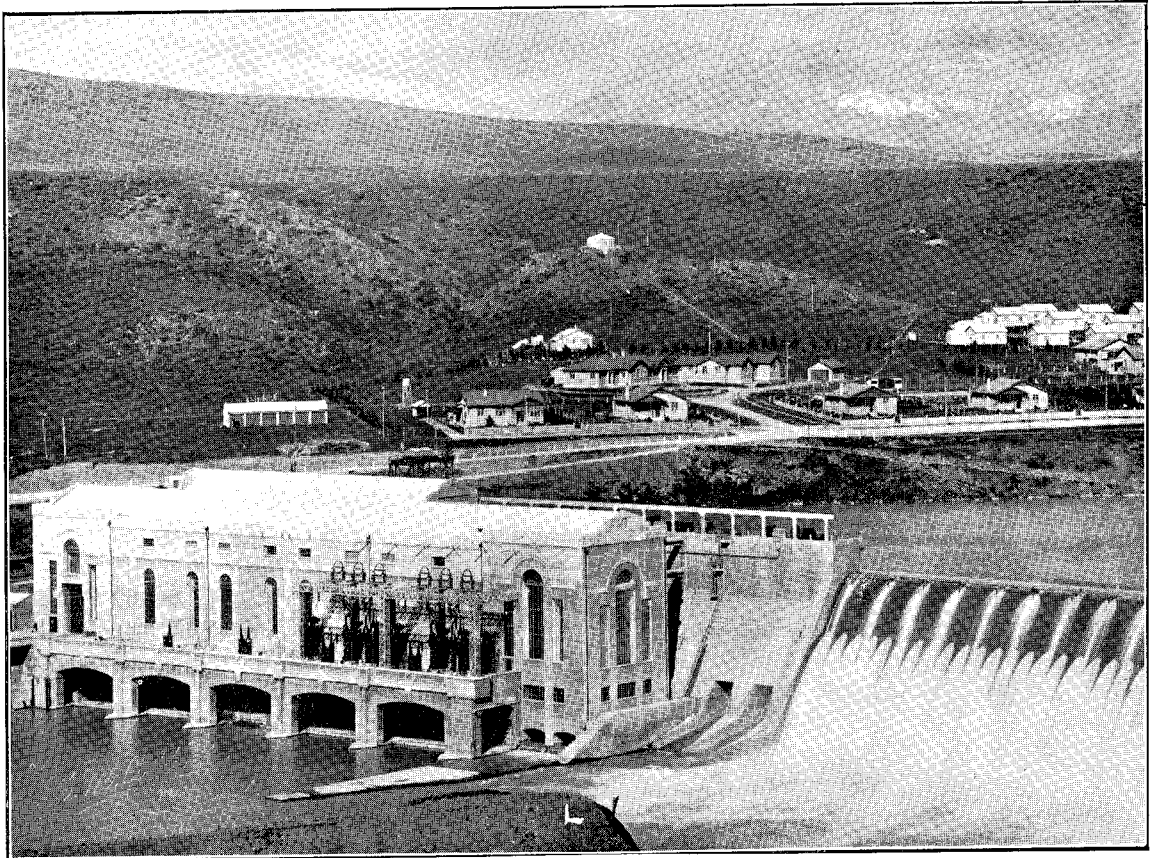
POWER-HOUSE AND PORTION OF DAM. WAITAKI POWER DEVELOPMENT.
