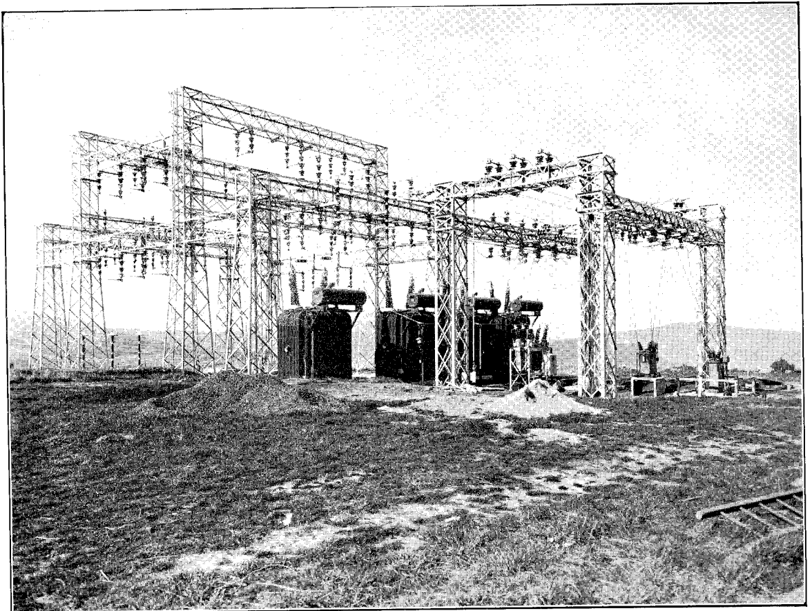
HALF-WAY BUSH SUBSTATION, DUNEDIN. WAITAKI POWER DEVELOPMENT.
