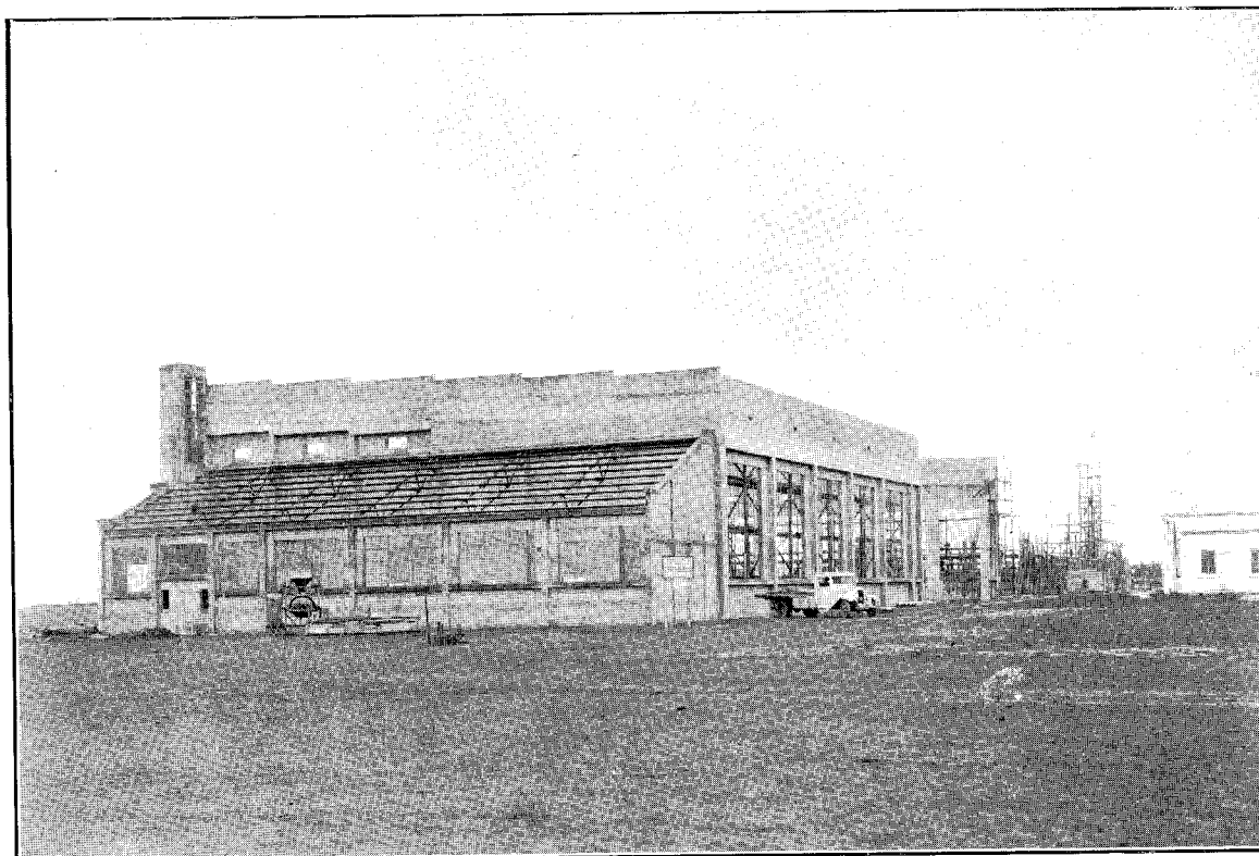
NOS. 1 AND 2 HANGARS UNDER CONSTRUCTION. WIGRAM AERODROME.
