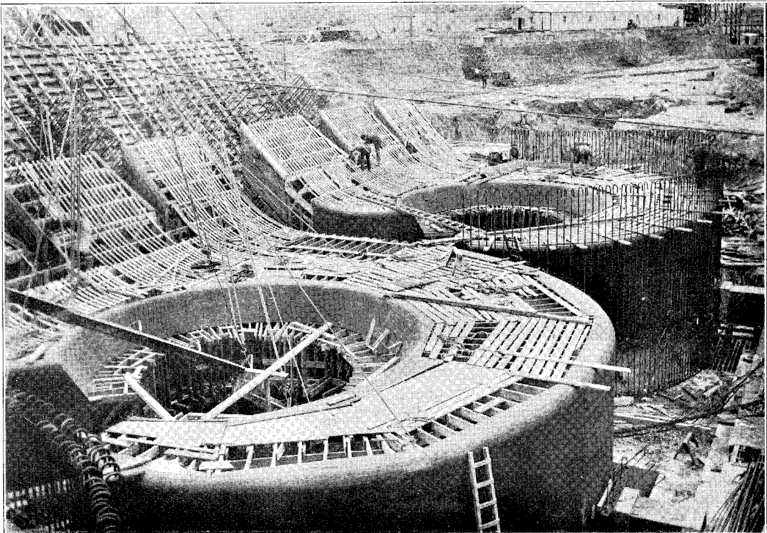
FORMWORK FOR PENSTOCKS AND SCROLL CASES FOR 20,000 H.P. TURBINES.
