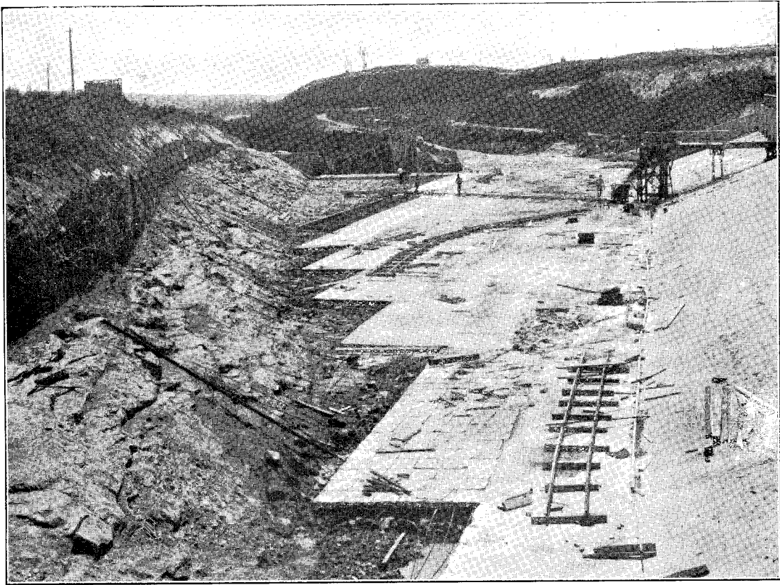
OVERFLOW-CHANNEL LINING BETWEEN SPILLWAY EXTENSION AND DROP WEIR.
