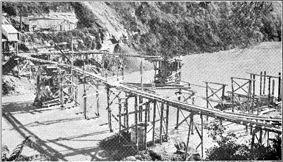
CYLINDER PIERS IN RIVER.
