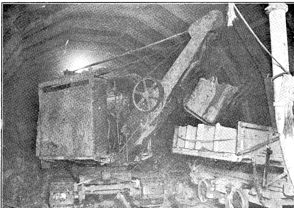
LARGE COMPRESSED-AIR SHOVEL IN NO. 2 TUNNEL.
