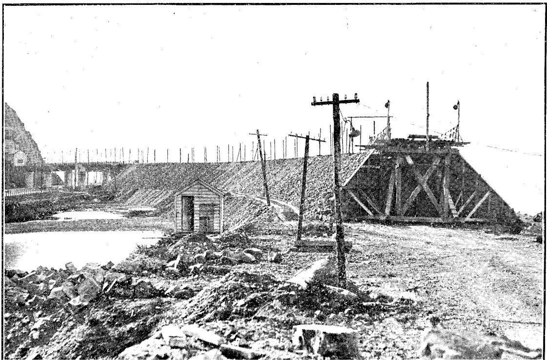
APPROACH BANK TO NO. 1 TUNNEL.—MOVABLE TREESTLE IN FOREGROUND.
