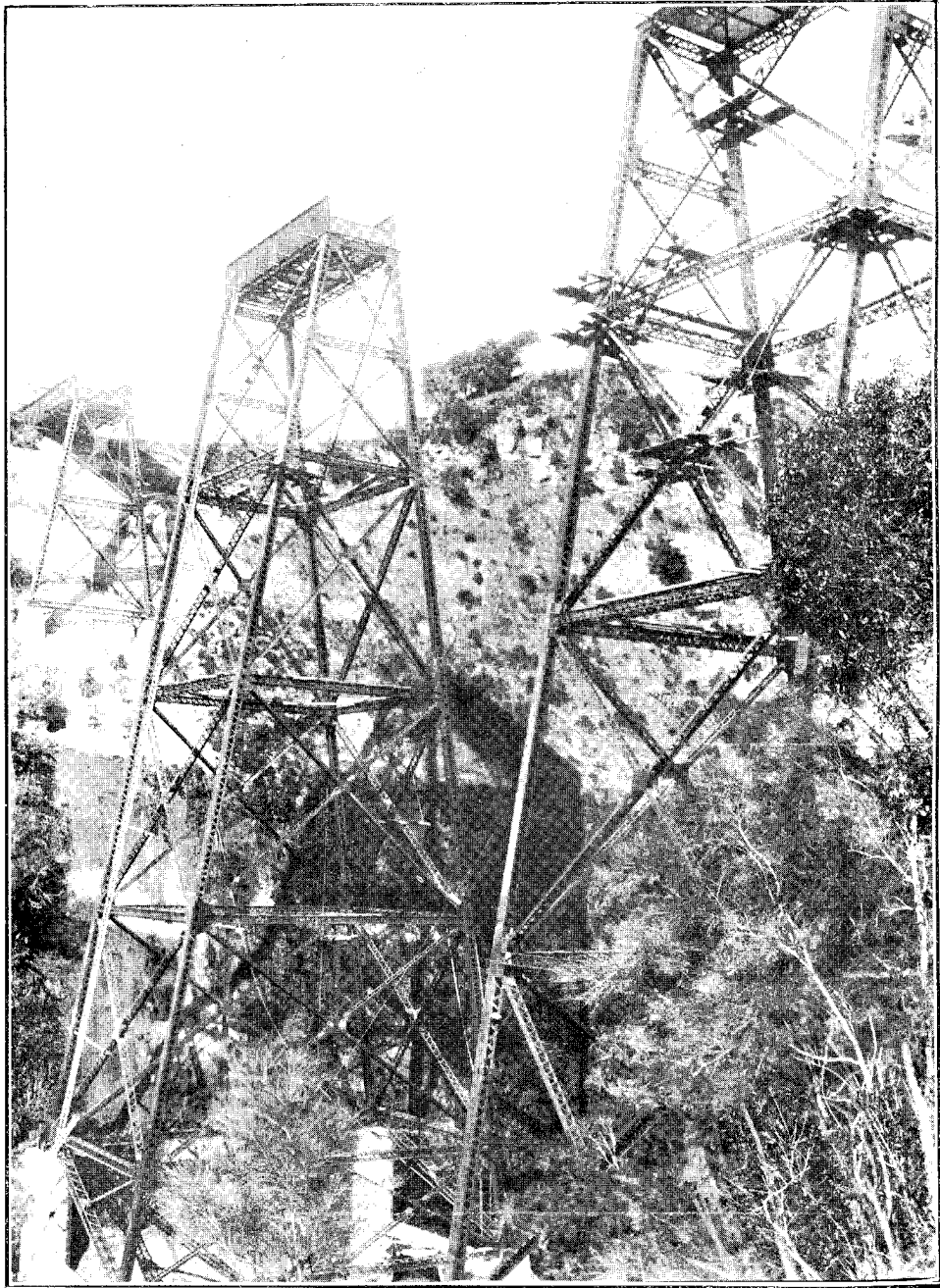
WAIKARE VIADUCT.—GENERAL ELEVATION OF MAIN TOWERS.
