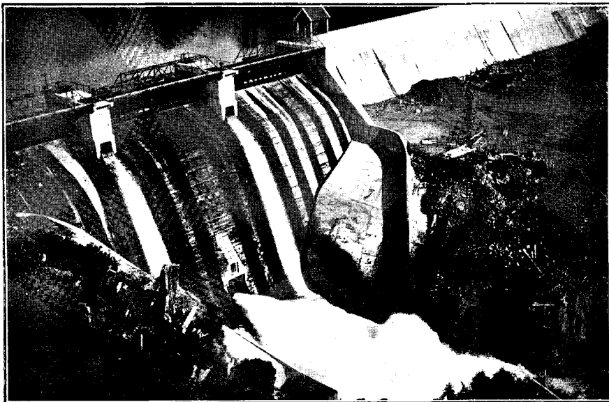
NO. 3 DAM, SHOWING DISCHARGE FROM REGULATING-JET DISPENSER. MANGAHAO POWER DEVELOPMENT.
