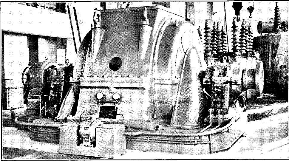
10,000 k.v.a. SYNCHRONOUS CONDENSOR.
