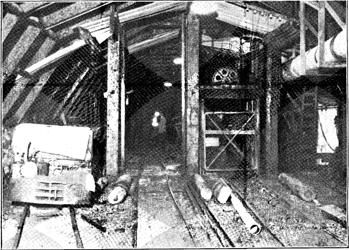
BOTTOM OF SHAFT OF NO. 2 TUNNEL, LOOKING TOWARDS WELLINGTON.
