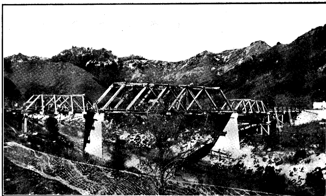
WAITOTARA RIVER BRIDGE, WAITOTARA VALLEY ROAD. (Main span, 120 ft.)
