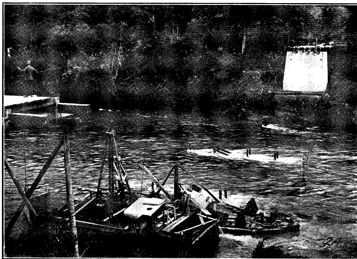
TE MAIRE BRIDGE, WANGANUI RIVER (8 M. BELOW TAUMARUNUI), UNDER CONSTRUCTION. View showing cofferdam for one of the main piers.
