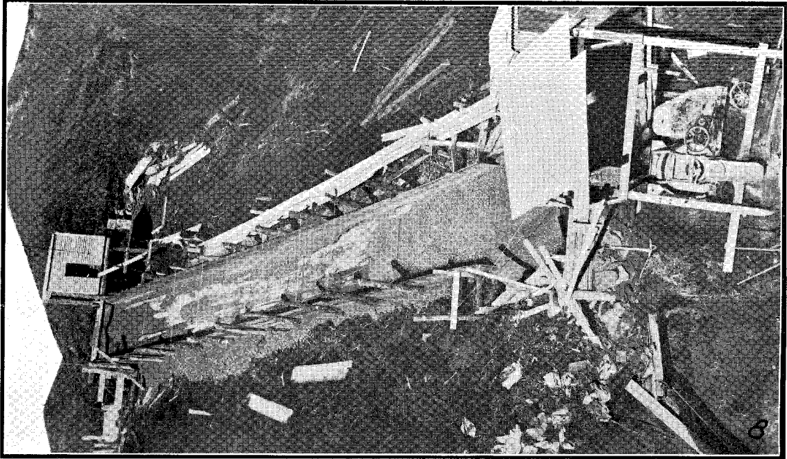
CHIMNEY CREEK TUNNEL No. 2, AT 47 M. 17 CH. North end concreting layout.
