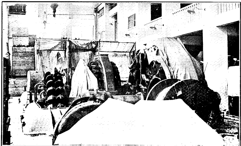
MANGAHAO HYDRO-ELECTRIC-POWER PLANT. MANGAHAO POWER-HOUSE: MACHINERY IN POSITION IN POWER-HOUSE, COVERED TO KEEP OUT DUST.
