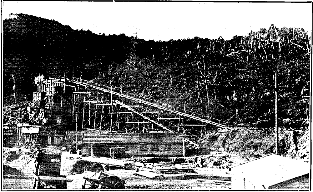
MANGAHAO HYDRO-ELECTRIC-POWER PLANT. CRUSHING AND CONCRETING PLANT, ARAPETI DAM.
