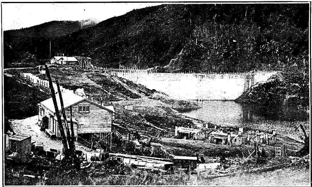
MANGAHAO HYDRO-ELECTRIC-POWER PLANT. WATER RISING IN RESERVOIR, ARAPETI DAM.
