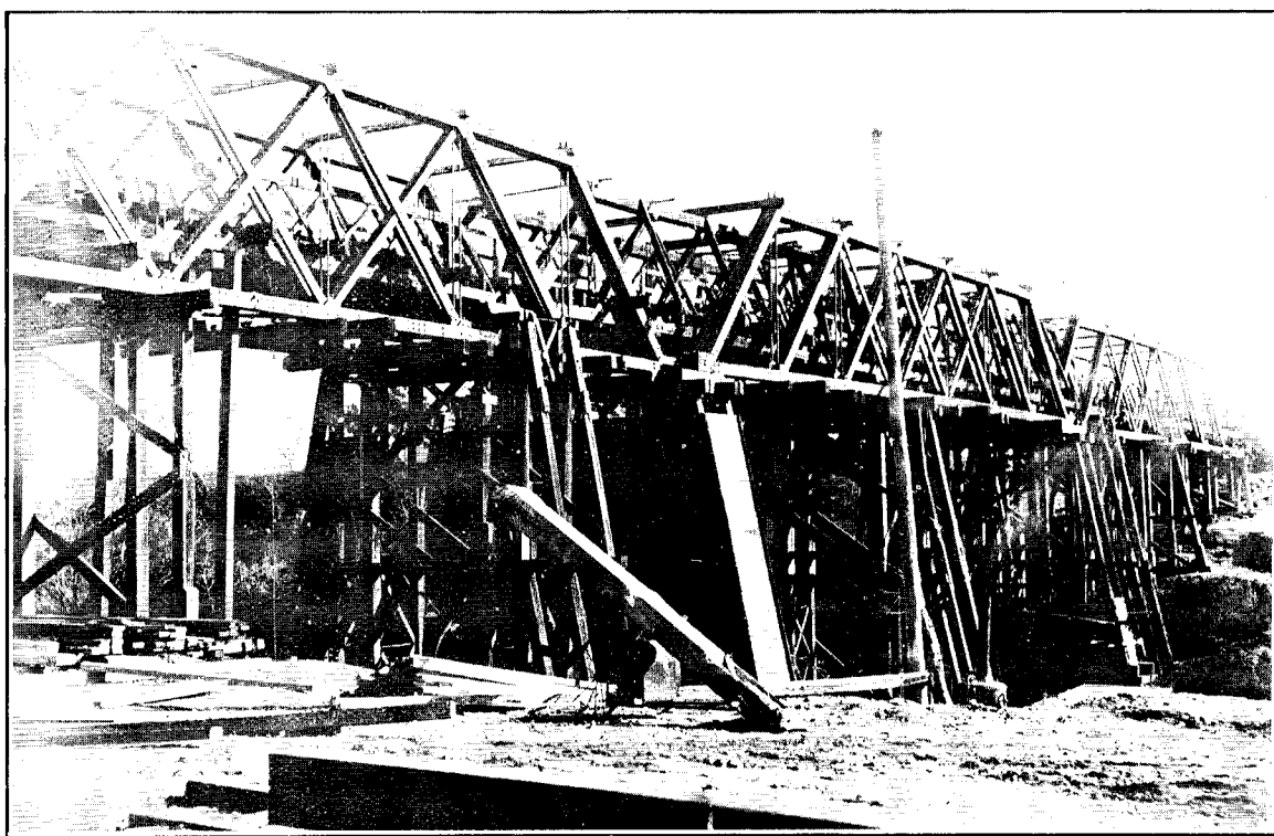
WAIPA RIVER ROAD-BRIDGE. WHATAWHATA : DETAIL OF CONSTRUCTION.
