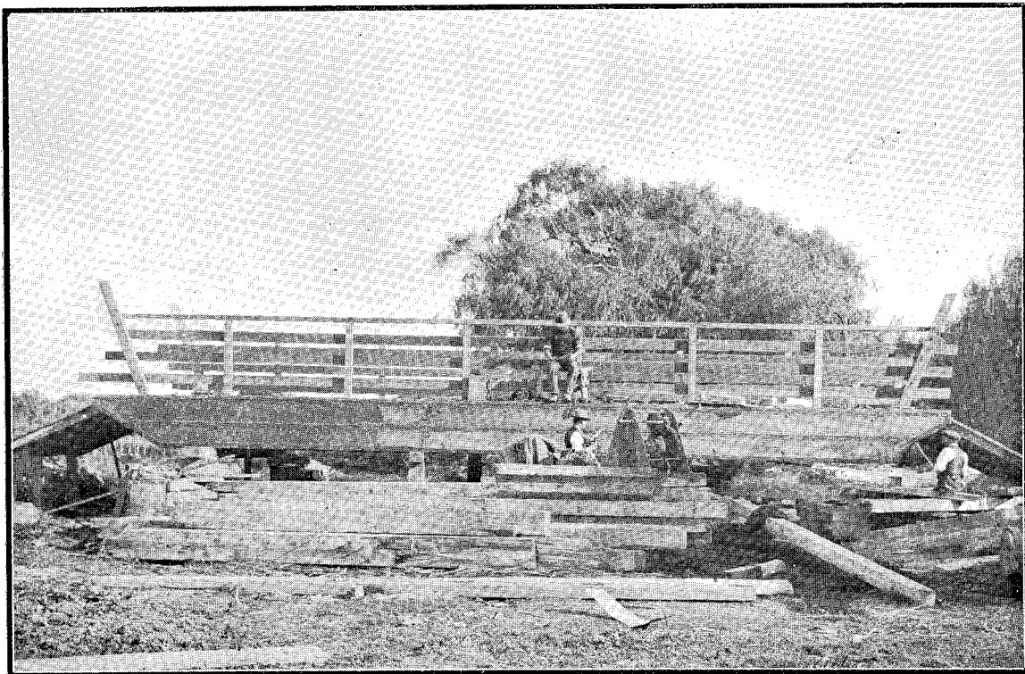
BUILDING FERRY PUNT FOR RIVER-DIVERSION.
