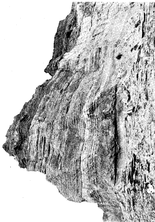
No. 8. COASTAL CLIFF NORTH OF WANGANUI, NEAR THE OTOTOKA STREAM.
