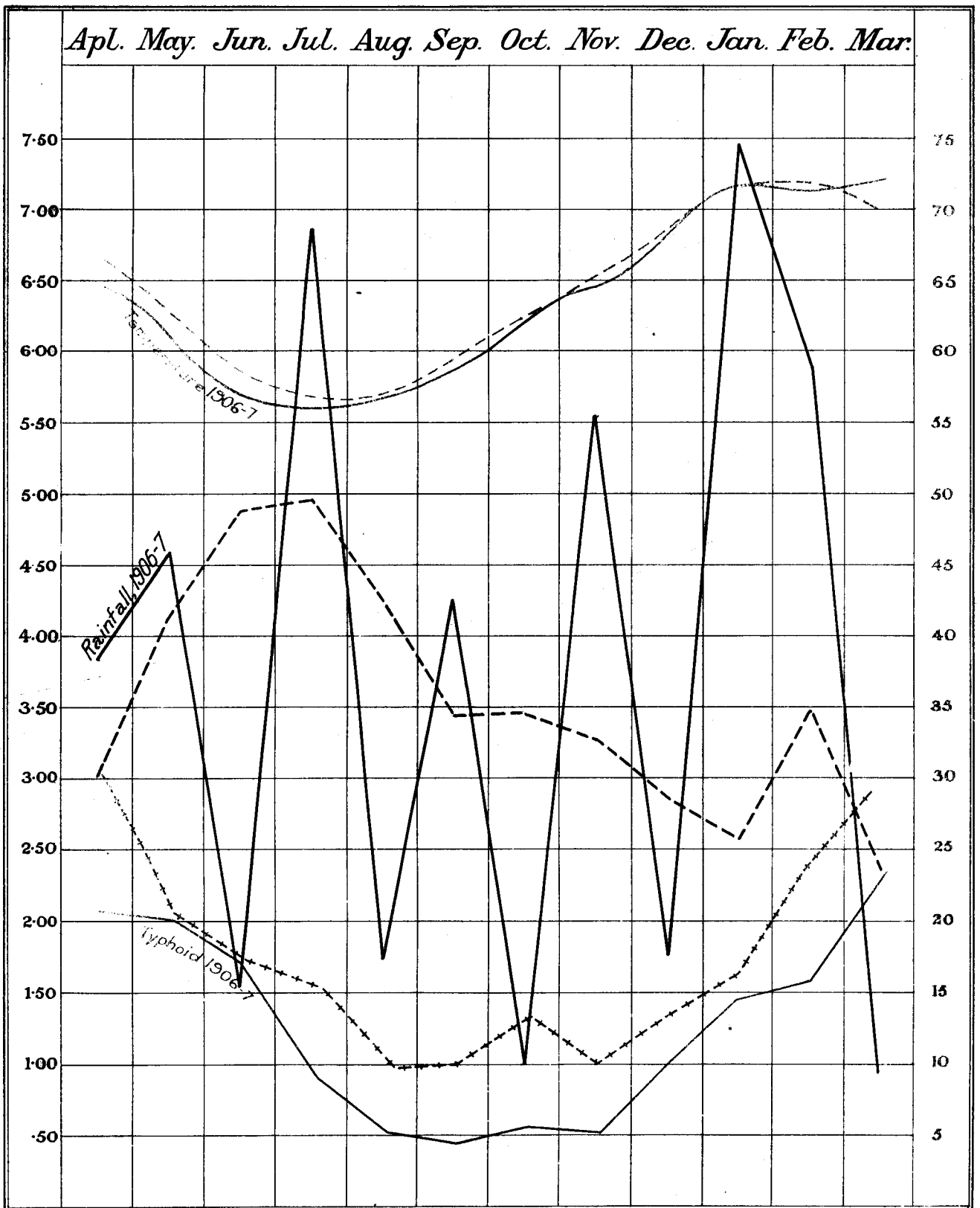
CHART A.—Showing TYPHOID, TEMPERATURE, and RAINFALL Curves, April, 1906, to March, 1907.
