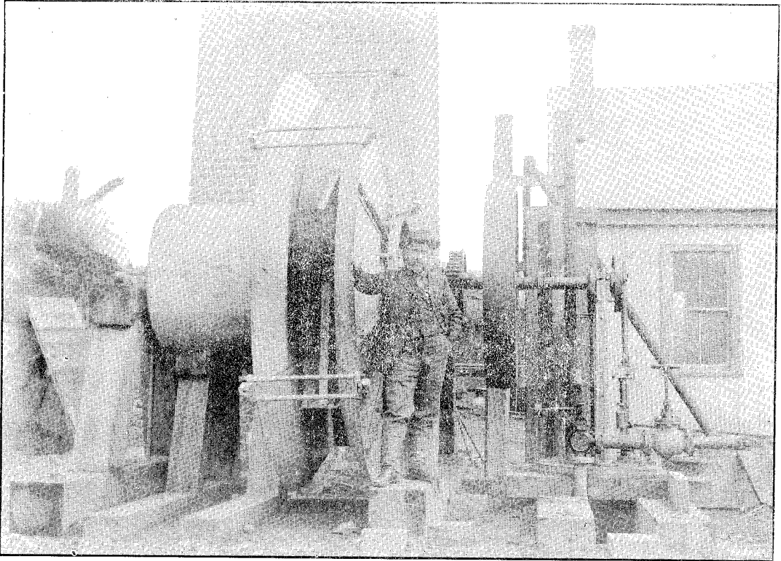
Ventilating Fan at Orepuke Shale-mine, Southland.
