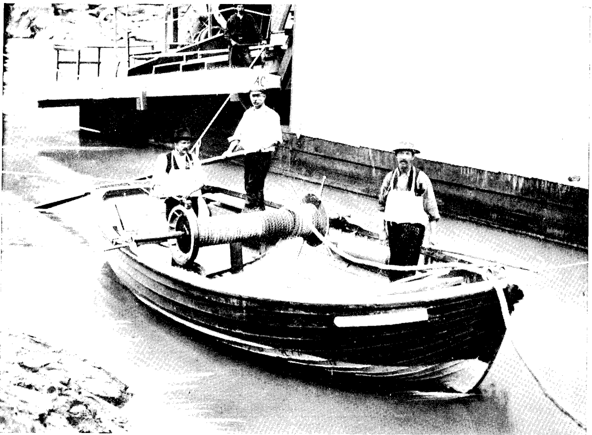
T. Shore's Arrangement of Reel for paying out Lines, Alpine Consols Dredge, Cromwell Gorge, Clutha River.
