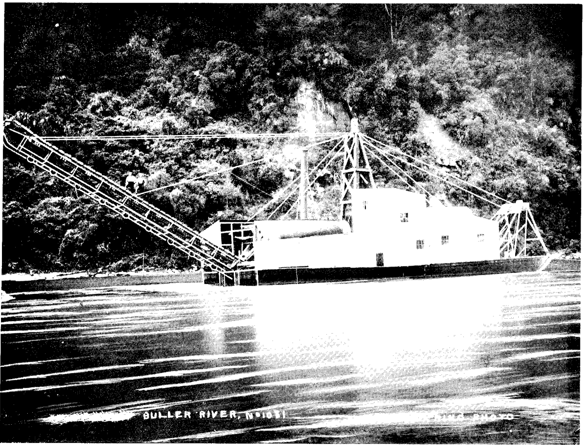
Buller Junction Dredge.
